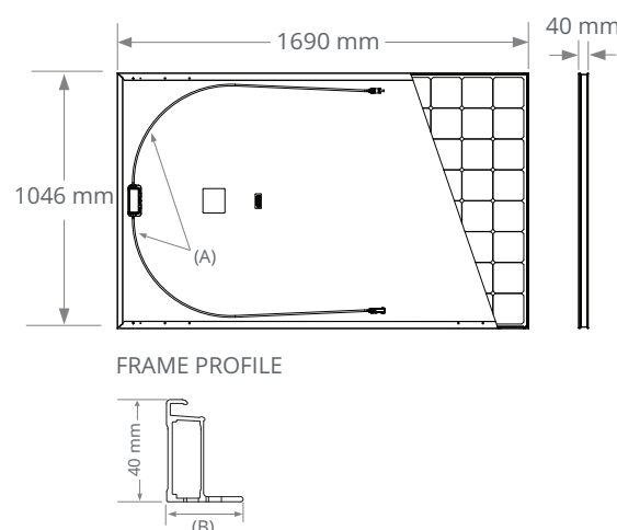
FRAME PROFILE A. Cable Length: 1200 mm +/-10 mm B. LONG SIDE: 32 mm SHORT SIDE: 24 mm
