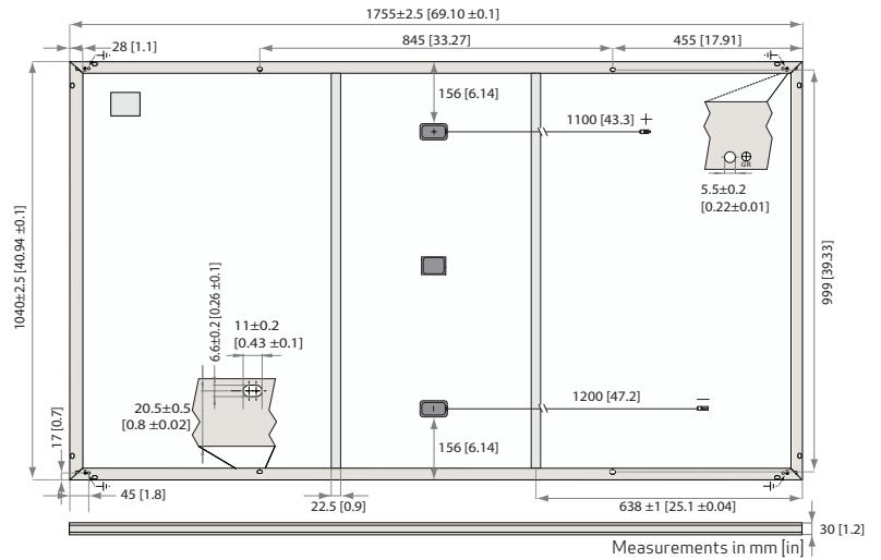
Fig. 22: Panel dimensions: REC TwinPeak 4 Series
