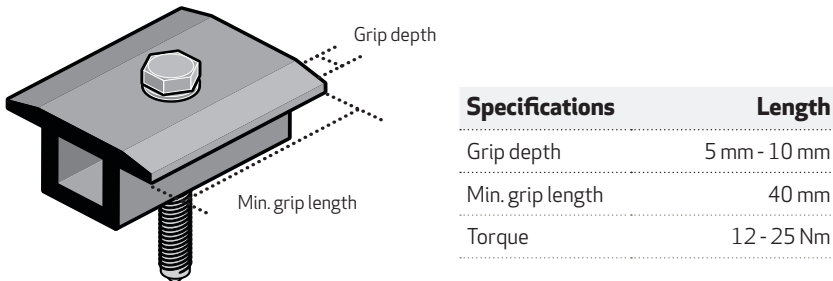
Fig. 1: Clamp specifications
