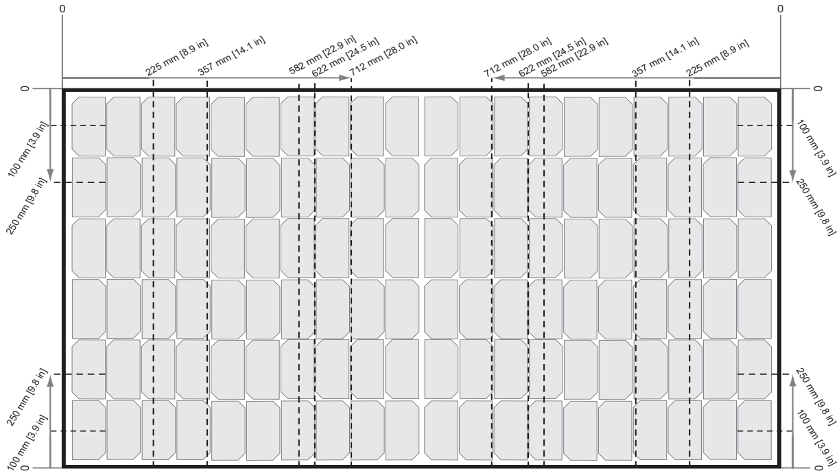
Fig. 11: Clamping of REC N-Peak 2 Series panels using short rails
