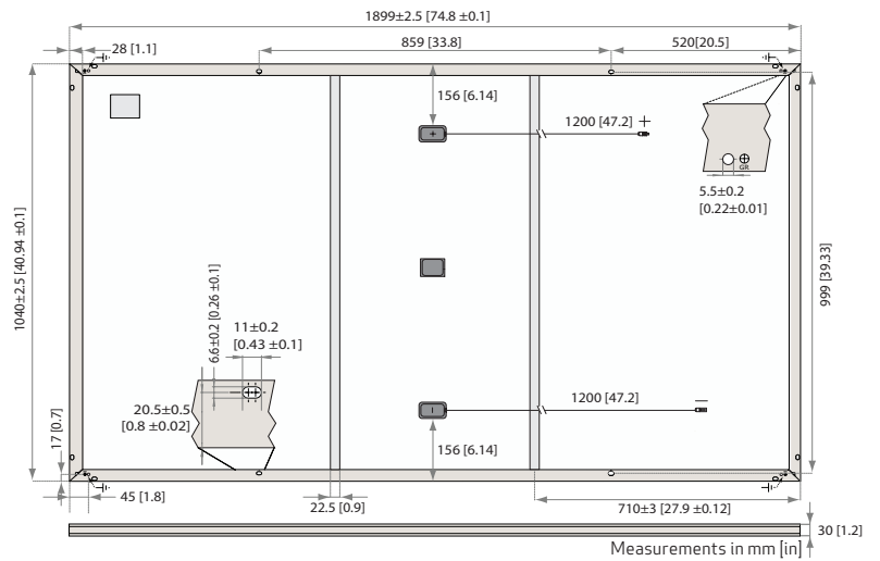
Fig. 24: Panel dimensions: REC TwinPeak 5 Series
