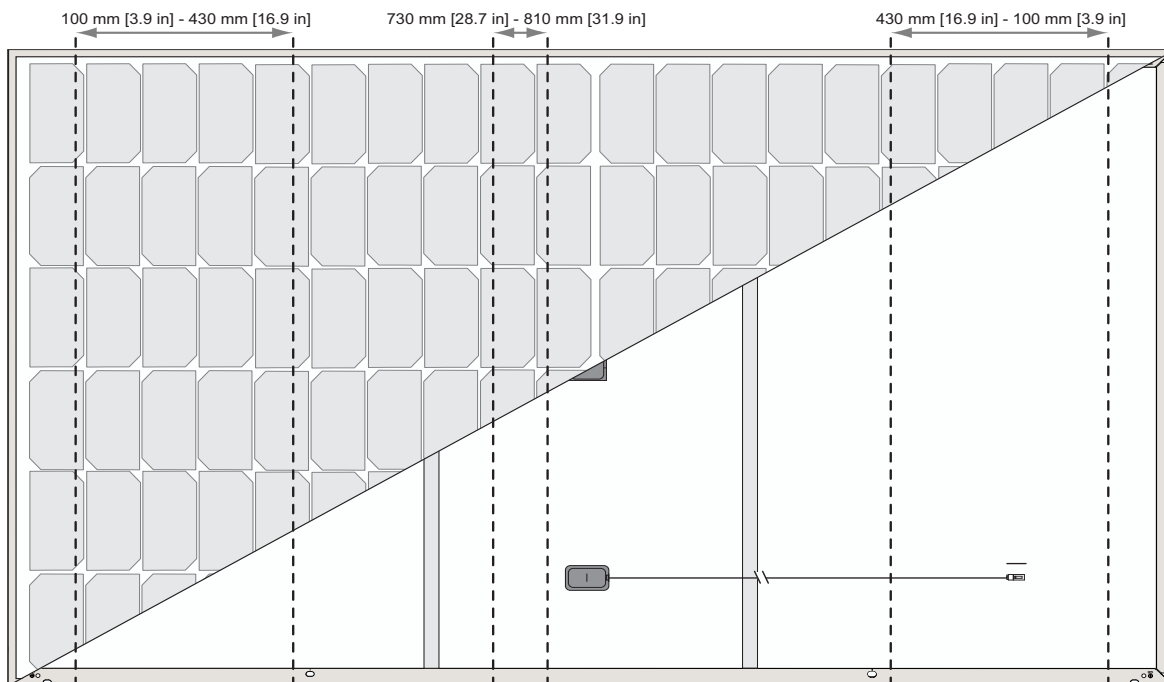
Fig. 18: Six-point mounting configuration clamping zones
