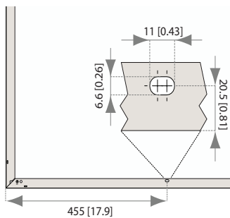
Fig.15: Mounting holes
