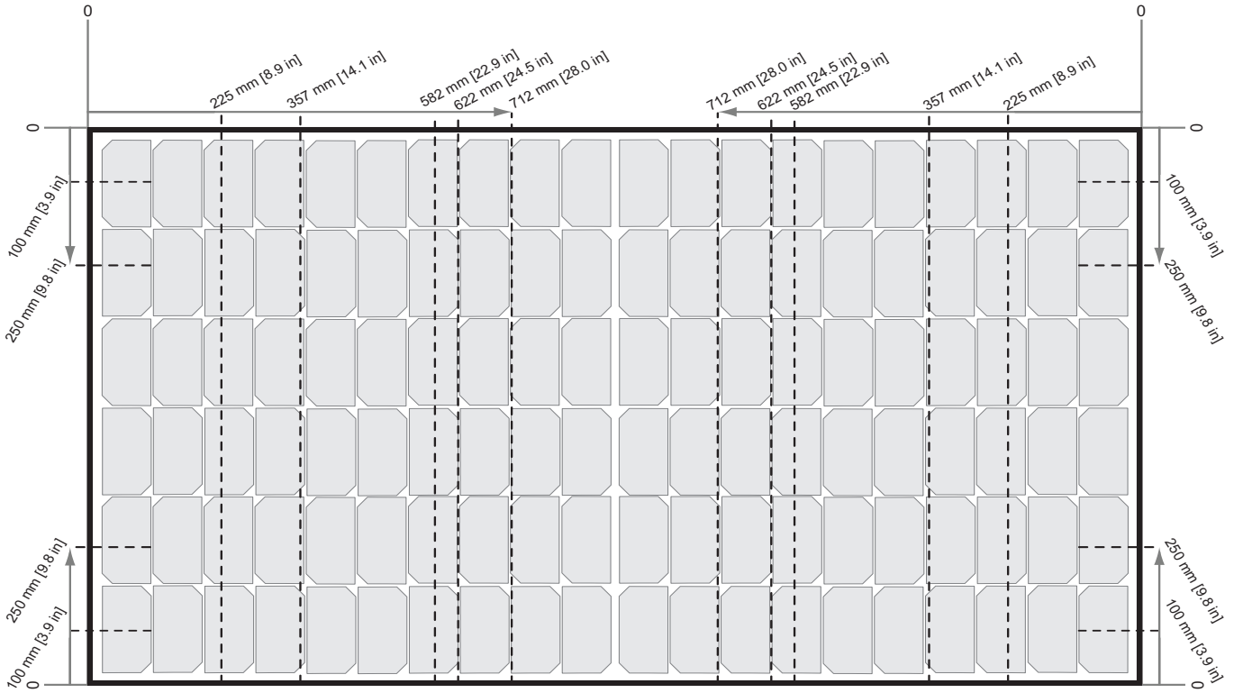
Fig. 9: Clamping of REC N-Peak 2 Series panels with rails parallel to short side of the panel
