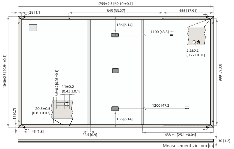
Fig. 23: Panel dimensions: REC TwinPeak 4 Black Series
