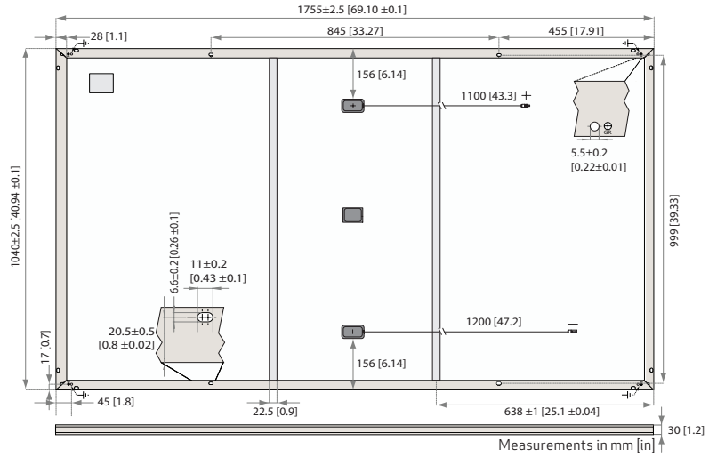
Fig. 26: Panel dimensions: REC N-Peak 2 Series
