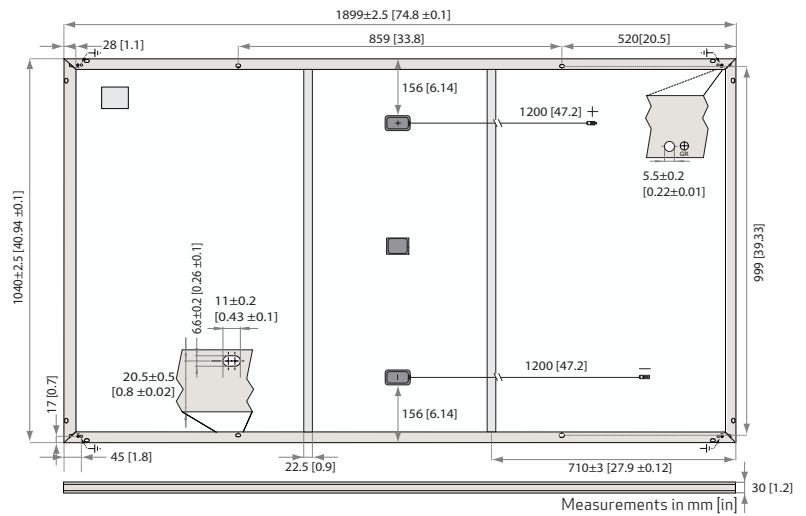
Fig. 25: Panel dimensions: REC TwinPeak 5 Black Series
