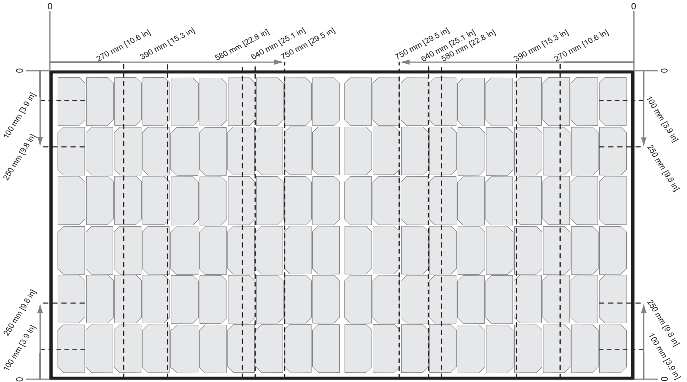
Fig. 6: Clamping of REC TwinPeak 5 Series panels with rails parallel to short side of the panel
