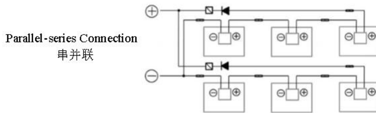
Fig. 5-6 Module connection method
