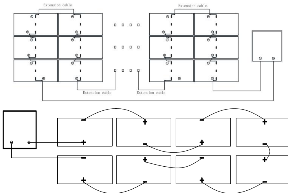
Fig. 5-5 Split J-Box at module middle position for horizontal direction
