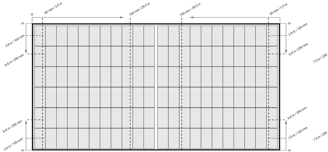
Fig. 2-2 Clamping of REC Alpha Pure 2 panels with Rails parallel to the Long Side of the Panel
