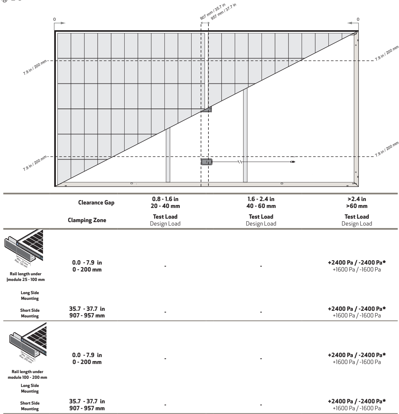
Fig. 2-5 Mixed Six-Point Mounting of REC Alpha Pure 2 Series Panels using short rails
