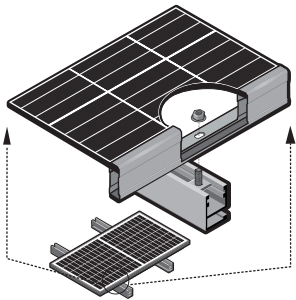
Fig. 1-4 Mounting holes: REC Alpha Panels
