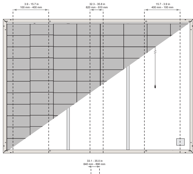
Fig. 4-2 Six-point mounting configuration clamping zones: REC Alpha Pure-RX
