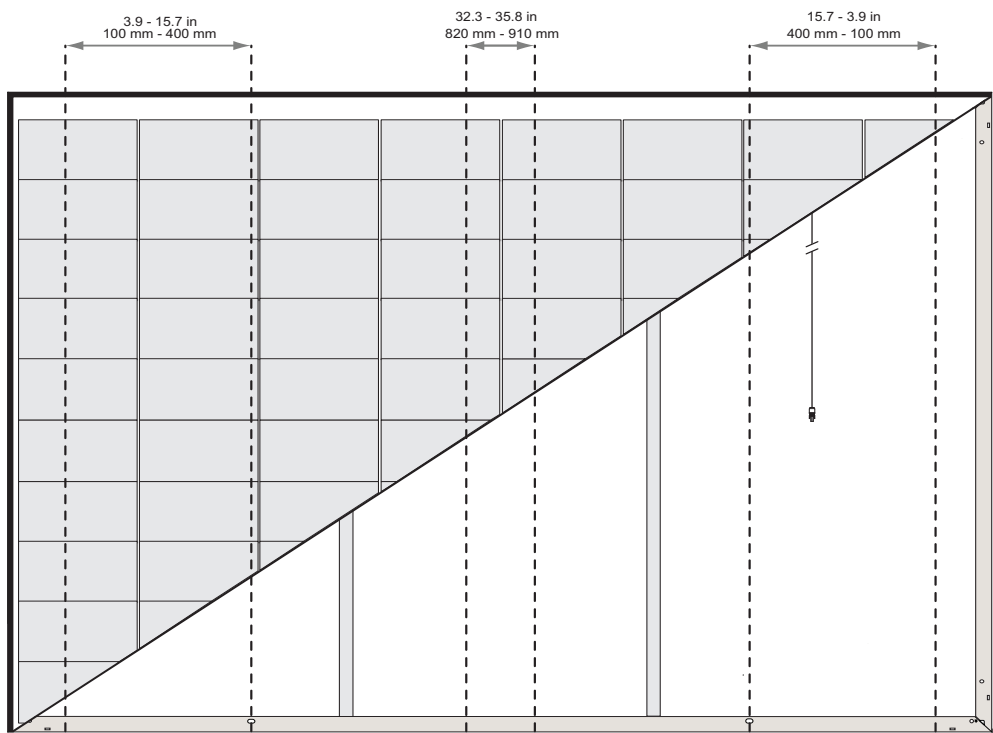
Six-point mounting configuration clamping zones: REC Alpha Pure-R
