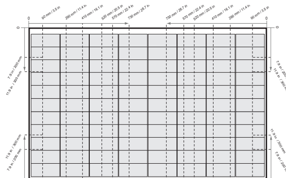
Fig. 4-1 Clamping of REC Alpha Pure-RX panels using short rails
