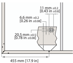
Fig. 1-5 Mounting hole installation example
