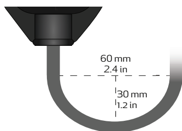
Fig. 1-7 Minimum Cable Distance
