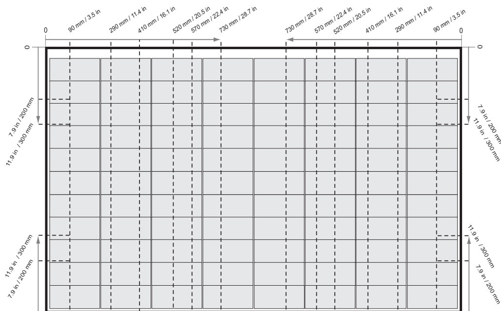
Fig. 3-3 Clamping of REC Alpha Pure-RX panels with Rails parallel to the Short Side of the Panel
