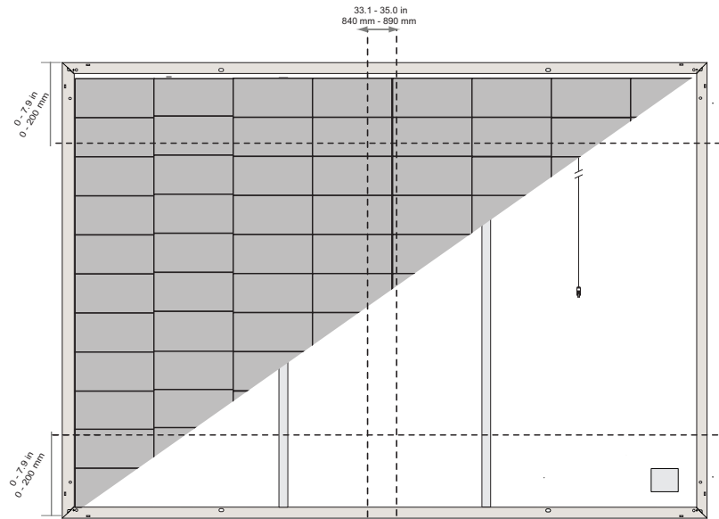
Fig. 4-3 Mixed Six-Point Mounting of REC Alpha Pure-RX Series Panels using short rails
