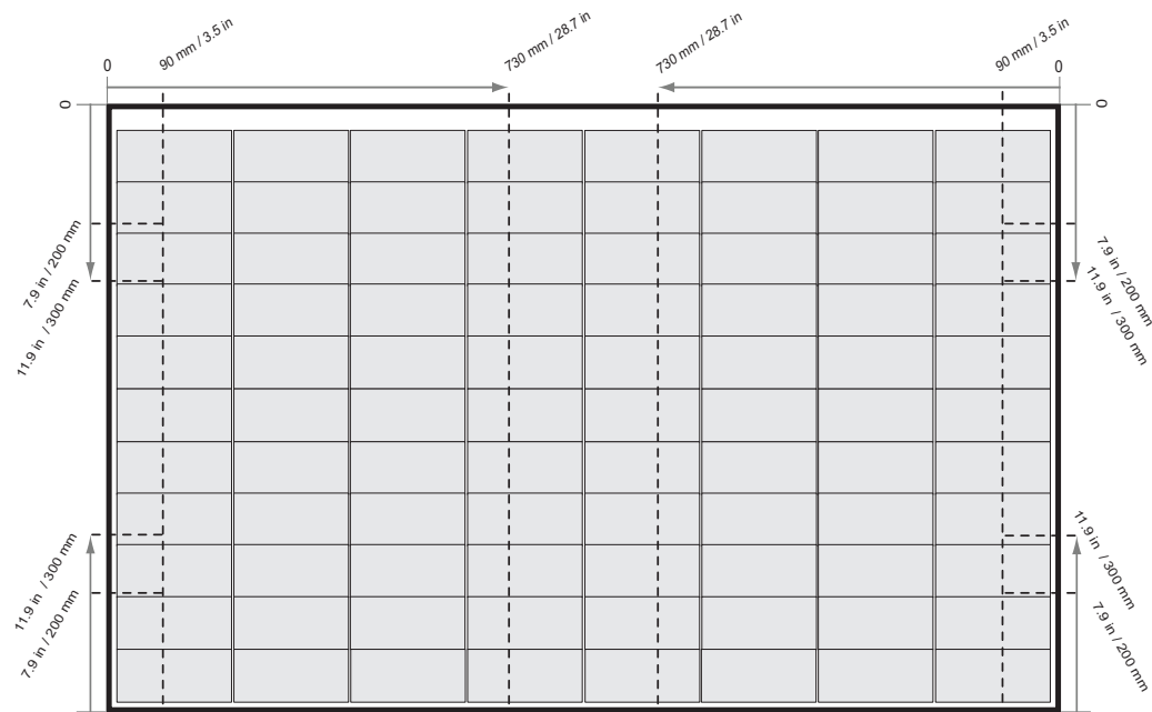
Fig. 3-4 Clamping of REC Alpha Pure-RX panels with Rails parallel to the Long Side of the Panel
