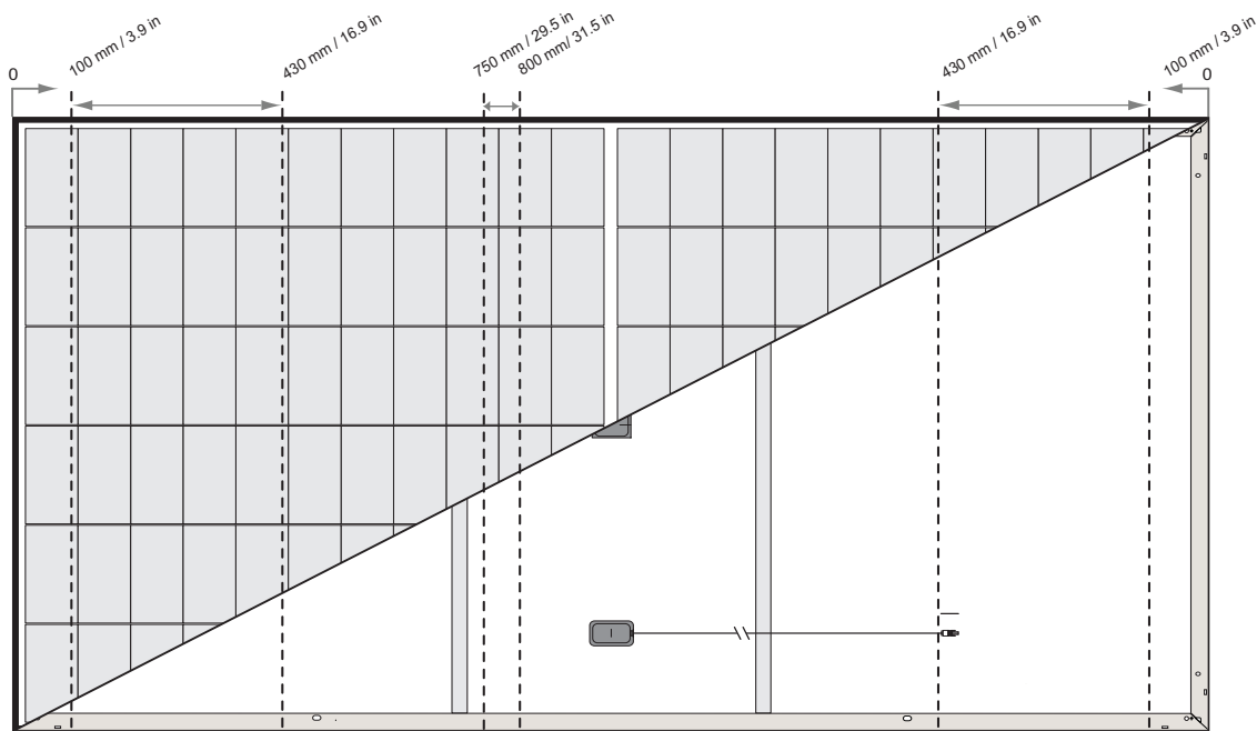
Fig. 2-4 Six-point mounting configuration clamping zones: REC Alpha Pure 2
