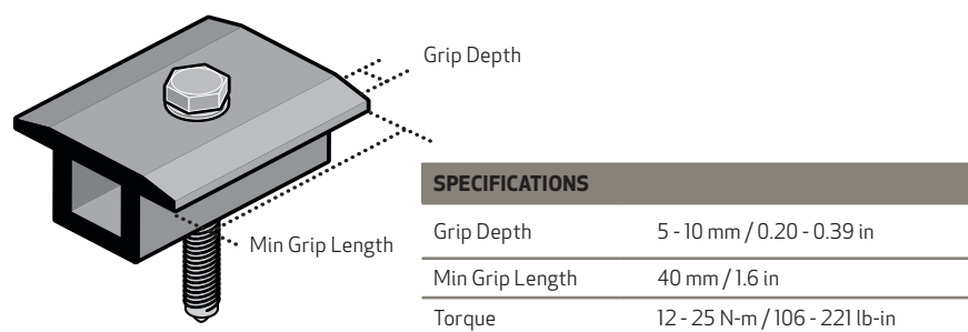
Fig. 1-1 Clamp Specifications
